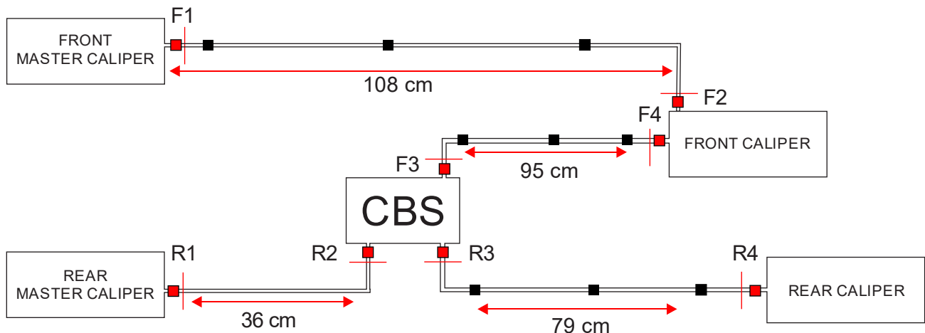
Gbr 3. Diagram Brake System ADV 160 CBS
