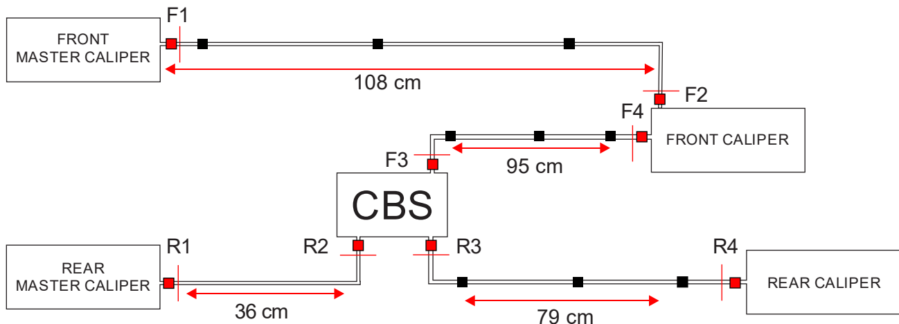
Pic 3. ADV 160 CBS Brake system Diagram
