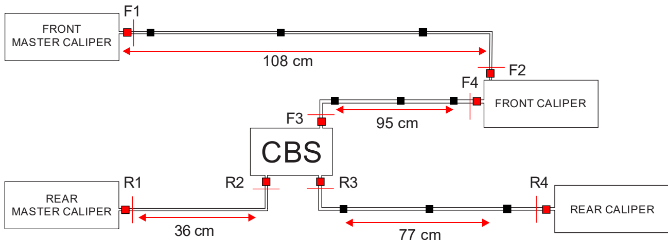
Pic 3. PCX 160 / New PCX 150 CBS Brake System Diagram
