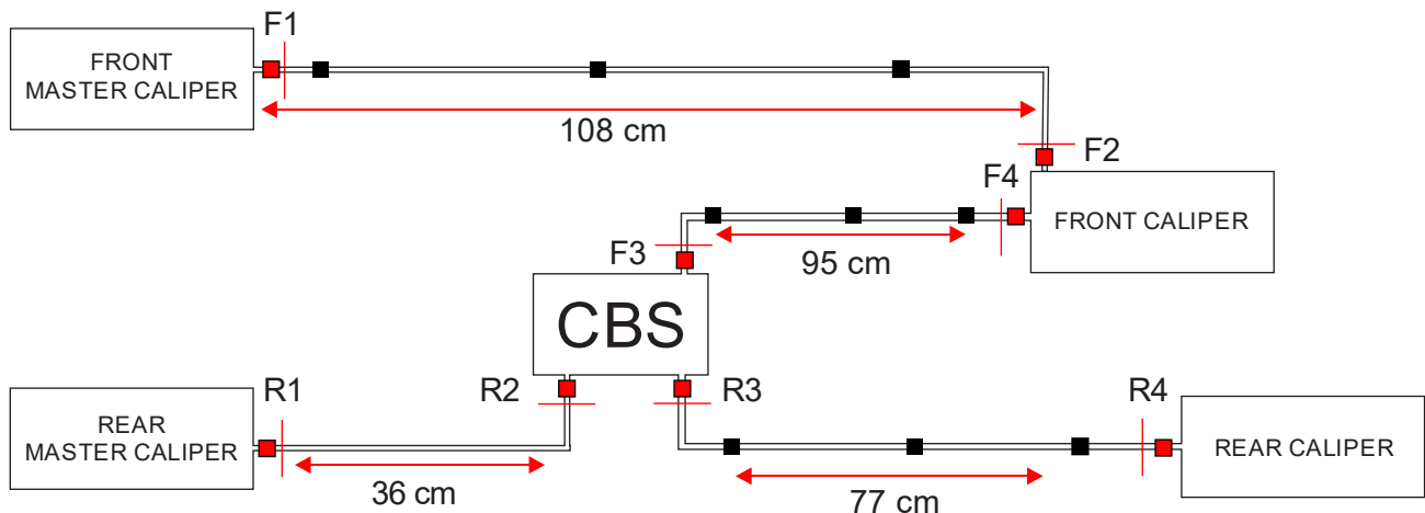
Gbr 3. Diagram Sistem Rem PCX 160 / New PCX 150 CBS
